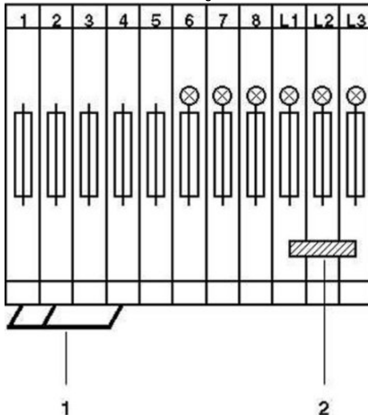
Circuit diagram
