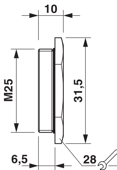
Dimensional drawing
