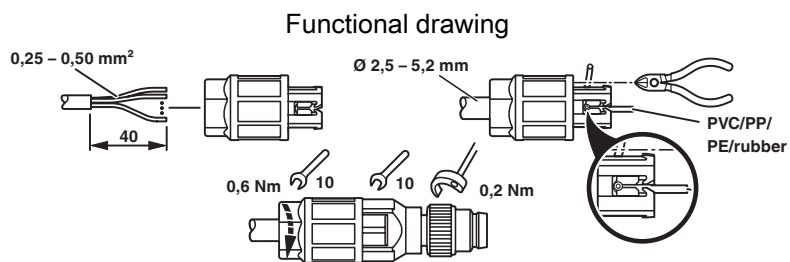
Pin assignment M8 plug, 4-pos., view male side
