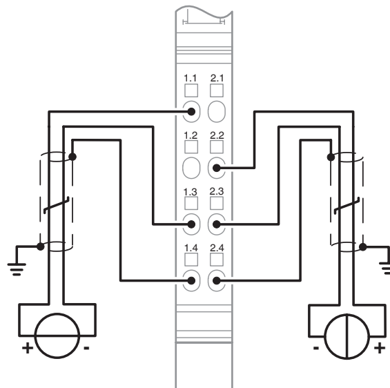
Connection diagram
