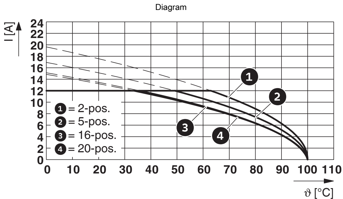
Type: FKCT 2,5/...-ST with MSTBVA 2,5/...-G
