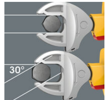
The corner-width rectangular prisms in the jaw allow a return angle of only 30°.
